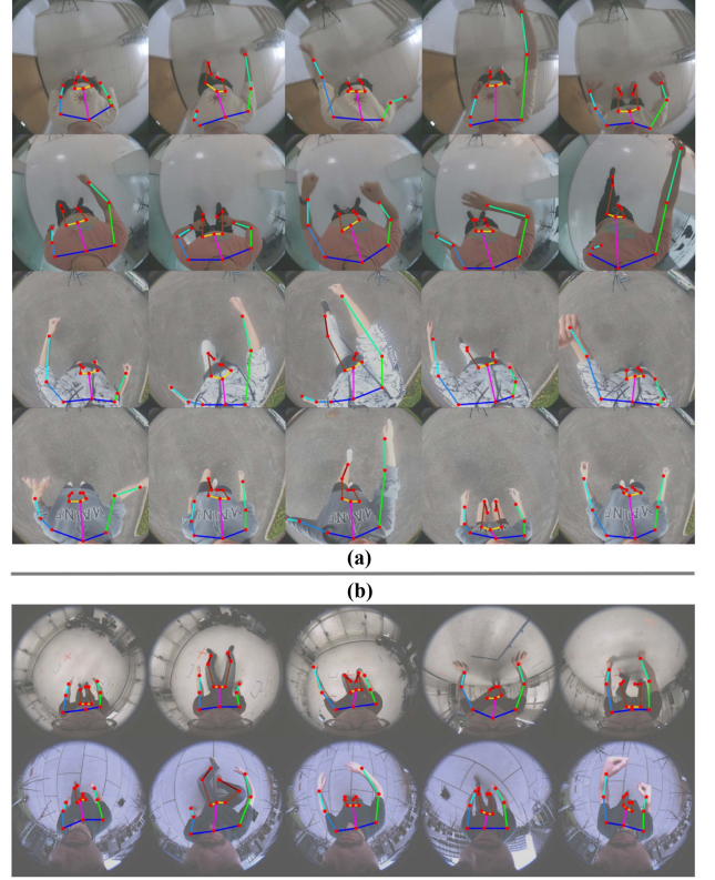
Fig. 7. Visualization results of egocentric 2D pose estimation by our proposed EgoFish3D. (a) On ECHP dataset; (b) On Mo 2 Cap 2 dataset. The red points are the predicted joint positions and the colorized lines indicate the skeleton.
