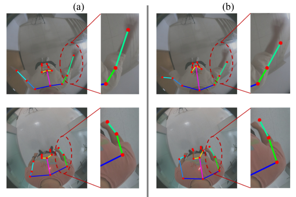
Fig. 8. Visualization of 2D pose by the proposed (a) egocentric module and (b) reprojection of the transformed 3D pose. The egocentric module can generate more accurate 2D pose than the reprojected one, especially for the joints of the upper limb.
