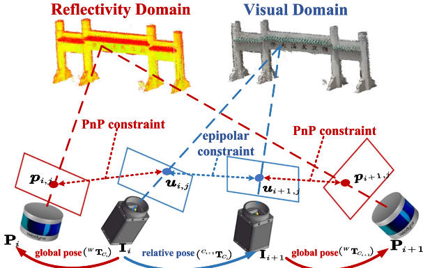
Fig. 5. Details of our proposed camera pose joint optimization framework.
