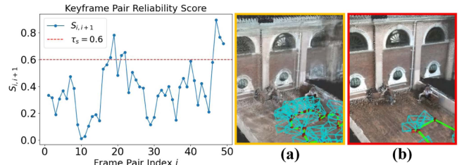
Fig. 8. The left figure shows reliable scores calculation. (a) shows the results without keyframe optimization. (b) shows the optimized result.
