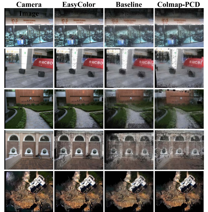
Fig. 10. Results of projecting colored point cloud generated by different methods on various public datasets onto image plane. Baseline result is obtained by coloring the point cloud using FastLIVO2 [6] and official extrinsic file. A manual 0.1 s time offset was added to ensure a fair comparison.
