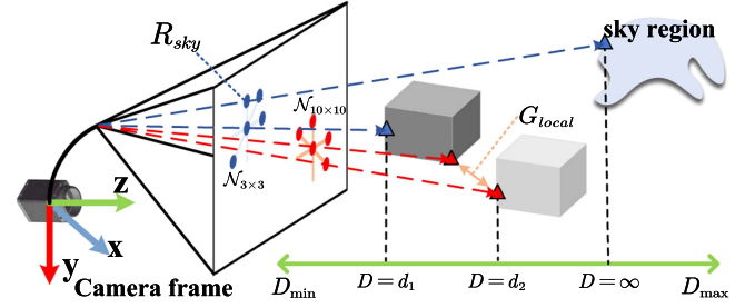
Fig. 6. Illustration of two types of unreliable edge region detection.
