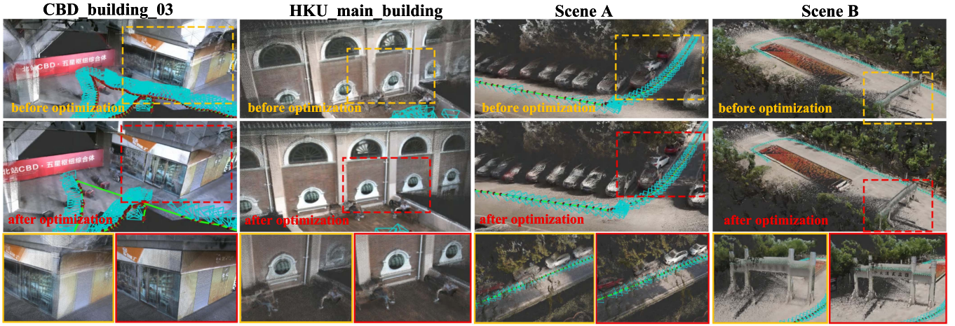
Fig. 11. Qualitative comparison of point cloud colorization results on FastLIVO2 dataset (CBD and main building sequence) and our self-recorded dataset (Scene A and Scene B). The reflectivity point cloud map for FastLIVO2 dataset is built using FastLIO2 [6], while the map for our dataset is generated with FastLIO2 [6] using our sensor suite (as shown in Fig. 9). Yellow boxes highlight unoptimized details. Red boxes highlight optimized details.
