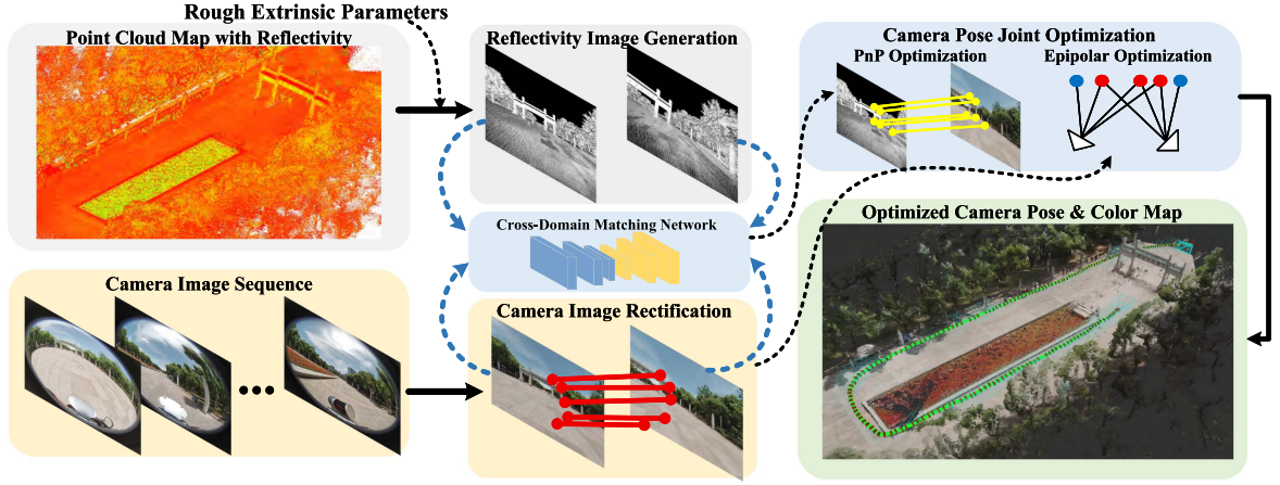
Fig. 2. Overview of the EasyColor framework. Given a pre-built point cloud map and an image sequence, we can get optimized camera poses and colorized point cloud map. The main technical modules include reflectivity image generation, cross-domain image matching, camera pose joint optimization, and point cloud colorization.
