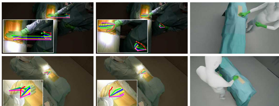
Fig. 1 Example showing the challenges of hand localization in surgical scenes caused by lighting conditions and the similar appearance of gloves and gowns. Left: RTMPose [1] fails to accurately localize the hands. Middle: our 2D predictions. Right: SMPL-X [2] 3D reconstruction using our 2D predictions from the same viewpoints
