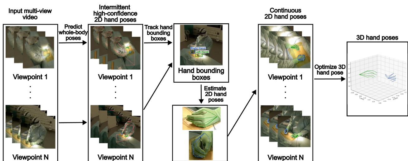
Fig. 2 Overview of our 3D hand pose estimation framework. Given multi-view videos from the OR, we first detect and track persons and then predict full-body and refined-body hand poses. Finally, we optimize a sequence of 3D hand poses consistent with anatomical and temporal constraints
