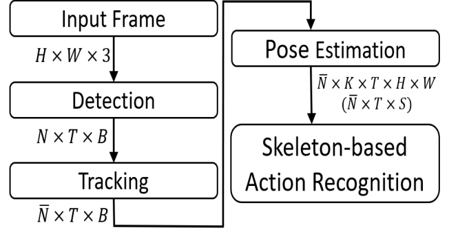
Figure 4: Overview of our real-world system for HPE. Depending on the interface of a following action recognition module, the output is either a 3D Heatmap Volume or a compressed skeleton abstraction
