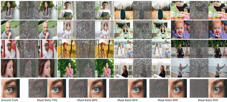
Fig. 3. In-the-wild generalization of Sapiens on unseen images. Top : Each triplet illustrates the ground truth (left), the masked image (center), and the MAE reconstruction (right), with a masking ratio of 75%, a patch size of 16, and an image size of 1024. Bottom : Varying the mask ratio between [0.75, 0.95] during inference reveals a minimal reduction in quality, underscoring the model’s robust understanding of human images.
