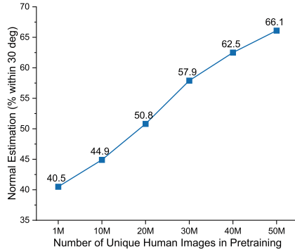
Fig. 10. Sapiens-0.3B’s normal estimation performance with unique human images seen during pretraining.
