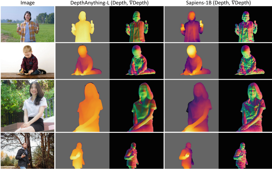
Fig. 8. We compare our depth prediction with DepthAnything [113]. To showcase the consistency of predicted depth, we also visualize the \nabla\text{depth} as pseudo surface normals.
