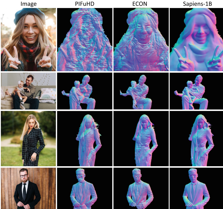
Fig. 9. Qualitative comparison of Sapiens-1B with PIFuHD [89] and ECON [108] for monocular surface normal estimation on challenging in-the-wild images.
