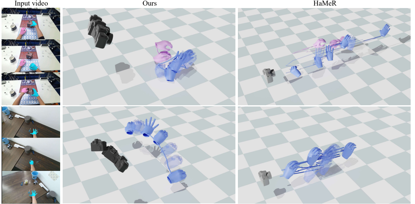
Figure 4. Qualitative comparison with state-of-the-art method HaMeR [37]. It can be seen that our method recovers significantly more plausible global hand motion. first row is from H2O dataset [21], while the second row is from HOI4D dataset [29].
