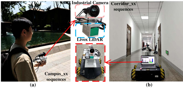
Fig. 5. Our platform with two usage configurations: (a) handheld and (b) robot-mounted. The LiDAR and the camera are hard synchronized with homogenous PWM signals.
