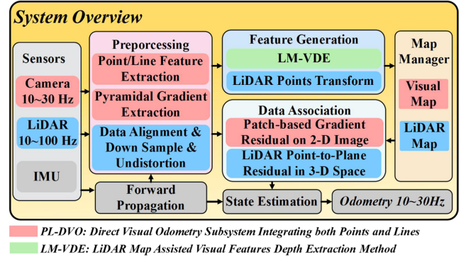
Fig. 2. System overview of the proposed PL-LIVO. This system comprises 4 basic modules: Preprocessing, Data Association, Feature Generation, and Map Manager. The measurements are fused based on an iterated error-state Kalman filter.
