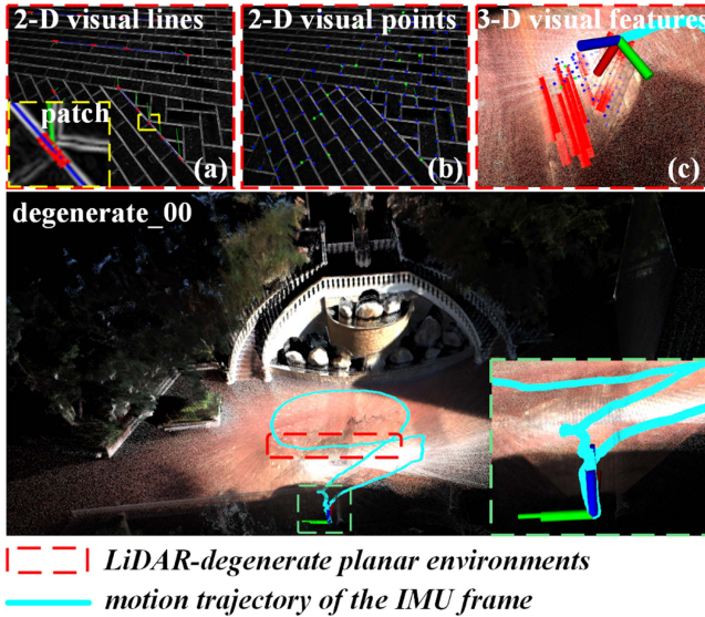
Fig. 6. Localization and mapping result of PL-LIVO under the degenerate_00 sequence. In this sequence, the LiDAR experienced degradation while oriented towards the ground. Due to the constraints provided by the gradient residuals of visual points and lines, PL-LIVO achieved stable localization and accurately returned to the origin.
