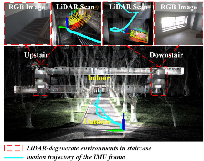
Fig. 1. localization and mapping result of PL-LIVO under the stairs_02 sequence. In this sequence, there was a significant exposure change when the operator entered indoors from outside. Moreover, challenging degeneration occurred when the operator was moving upstairs and downstairs, attributed to the limited FoV of the LiDAR scan.
