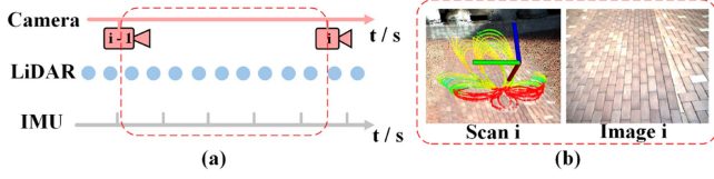
Fig. 3. Image-based Data Alignment. As (a) shows, the LiDAR scan is treated as a points stream (green and blue points from different scans). Points within the interval of two consecutive images (the red dotted box) are gathered as a new scan. As (b) shows, an aligned unit is generated with the new scan and the current image.
