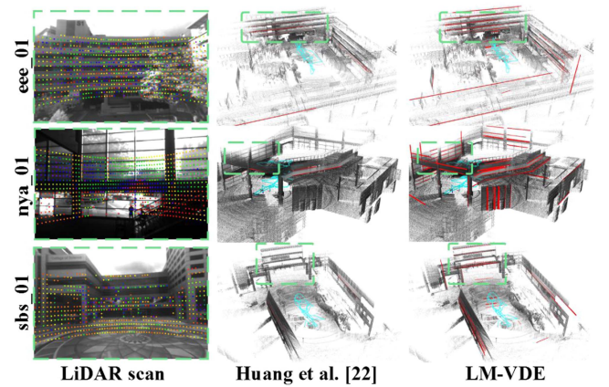
Fig. 7. Line map constructed by Huang et al. [16] and LM-VDE.
