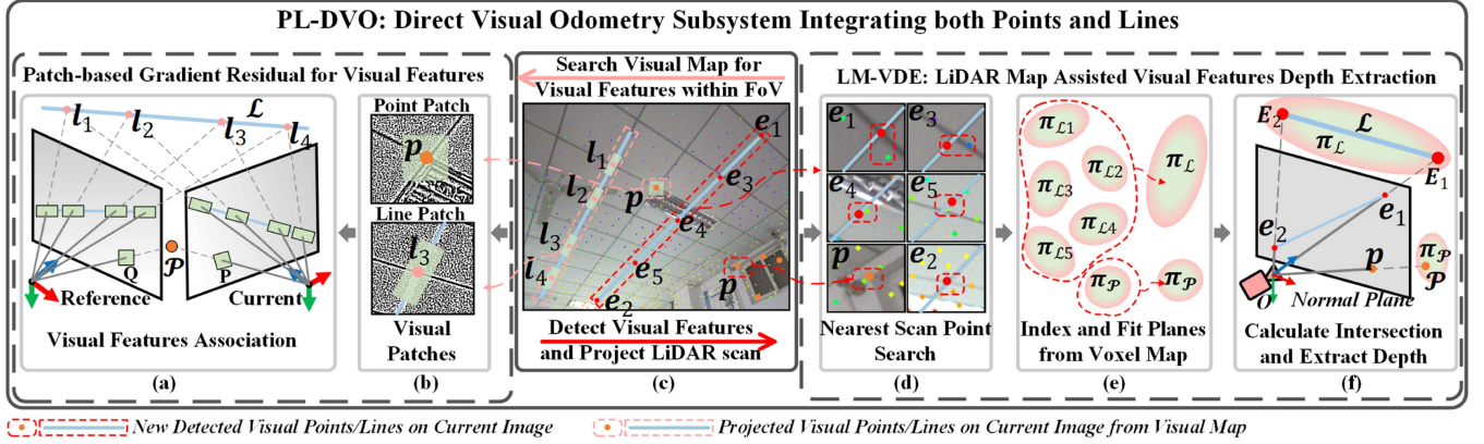
Fig. 4. Overview of the proposed PL-DVO. The proposed patch-based gradient residual for points and lines is constructed as (a). The utilized patch pattern is designed as (b). (c-f) depict the proposed LM-VDE method for extracting the depth of visual features.
