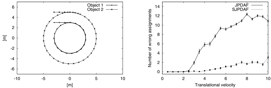
Fig. 14. Trajectory of two objects moving on concentric circles (left image) and average number of wrong associations depending on translational velocity (right image).
