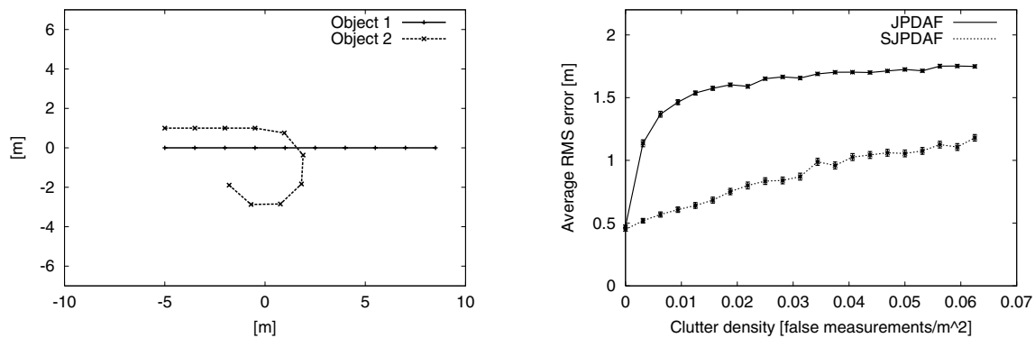
Fig. 15. Trajectory of the two objects being tracked (left image) and resulting average RMS error for increasing clutter densities (right image).
