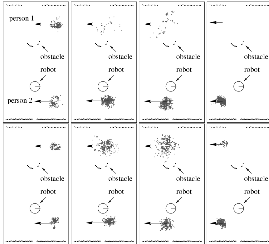
Fig. 16. Tracking two people with one sample set (top row) and with two sample sets (bottom row). The arrows indicate the position of the people and their movement direction.
