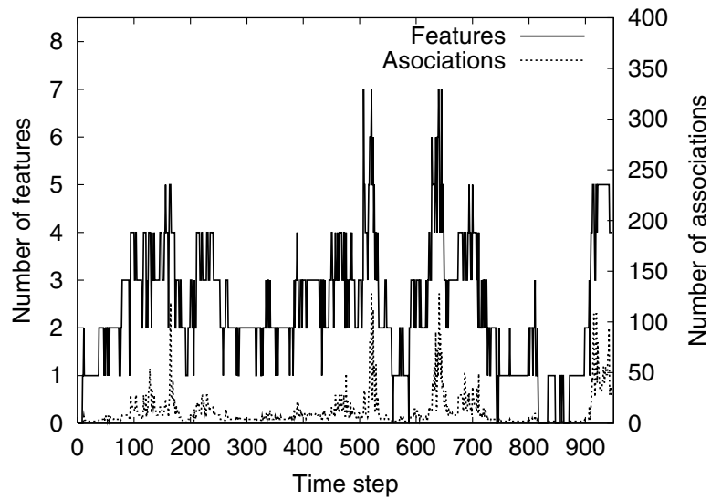
Fig. 7. The number of features detected in each scan of the experiment depicted in Figure 5 and the number of joint association events evaluated for each scan.
