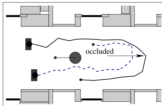
Fig. 11. Estimated trajectories of two people in a situation in which one person temporarily occludes the other. The arrow indicates the point in time when the occlusion occurred.
