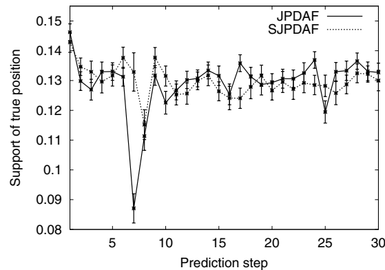
Fig. 13. Probability mass of the predicted state densities at the true locations of the object for the experiment illustrated in Figure 12. The false prediction of the Kalman filter leads to a low support at the true location.
