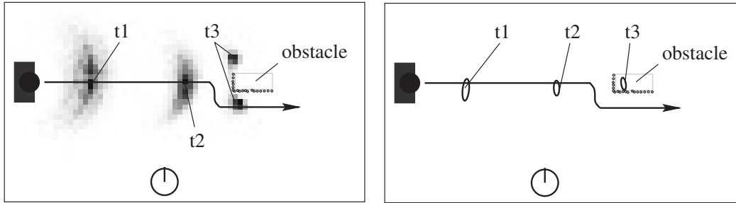
Fig. 12. Tracking one object approaching a static obstacle, using a particle filter (left) and using a Kalman filter (right). The arrow indicates the trajectory taken by the object. The Kalman filter erroneously predicts that the object moves into the obstacle.
