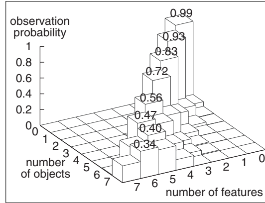
Fig. 1. The sensor model P(m_k | N^k) specifying the probability of observing m_k features, if N^k objects are in the perceptual range of the sensor.
