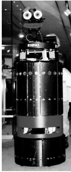
Fig. 2. The RWI B21 robot Rhino used for the experiments.
