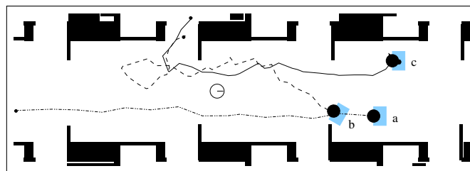
Fig. 9. Trajectories estimated by the SJPDF.
