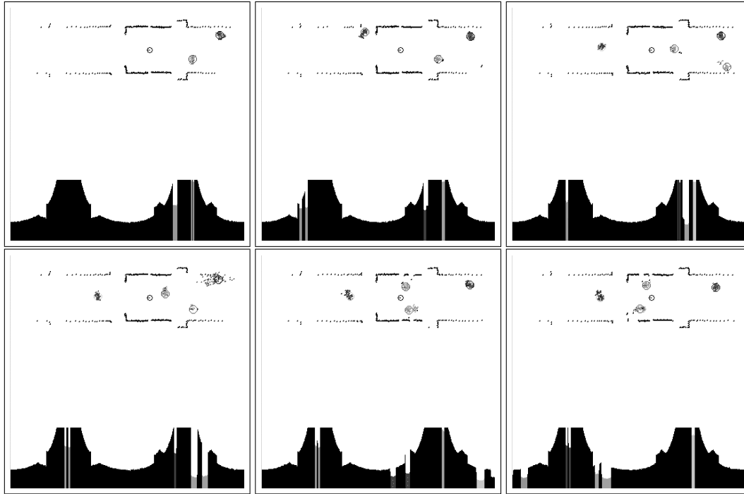
Fig. 6. Tracking people using laser range-finder data.
