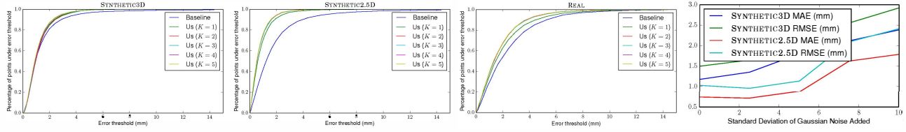
Figure 4. Left three panels: the percentage of data points whose error lies under a threshold for the baseline and our model with K basis components. Right: controlled noise experiments on the synthetic datasets.
