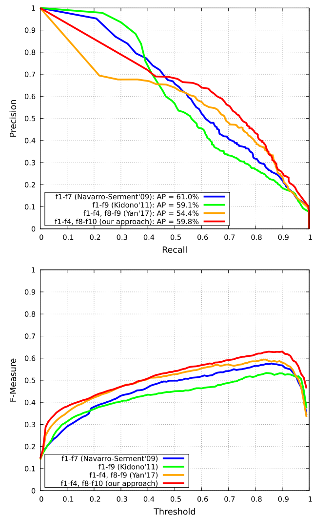
Fig. 16 Performance evaluation of different human classifiers
