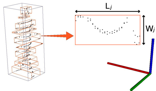
Fig. 6 The slice feature proposed by Kidono et al. (2011)
