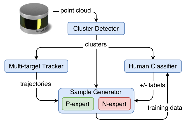
Fig. 2 Process details of the online learning framework
