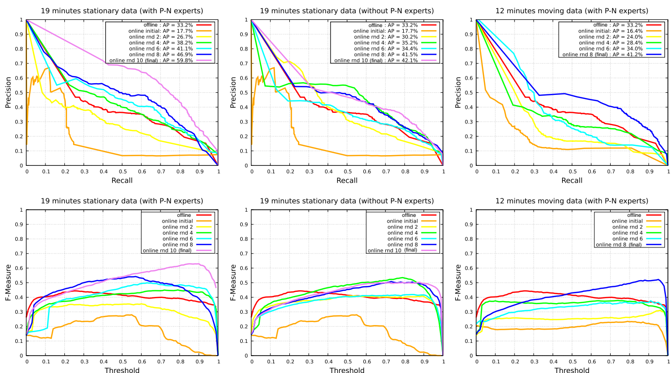
Fig. 15 Performance evaluation of the 3D LiDAR-based human classifier. Left column: online versus offline classification. Middle column: online classification without P–N experts. Right column: online clas-
