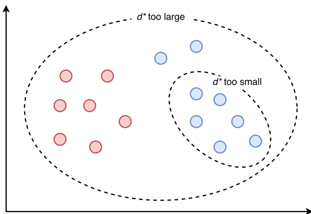
Fig. 3 Point cloud of two distinct objects (red and blue). Different values of d^* lead to different clustering results (Color figure online)
