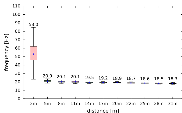
Fig. 12 Runtime performance of the clustering algorithm varying the maximum LiDAR detection range. For example, 2m refers only to the measurements (points) within this particular distance. The respective mean is shown on the top of each box. As one can see, the amount of clutter (and therefore detected clusters) is inversely proportional to the considered distance from the sensor. This is consistent with the complexity of the algorithm, i.e. \mathcal{O}(\log n)
