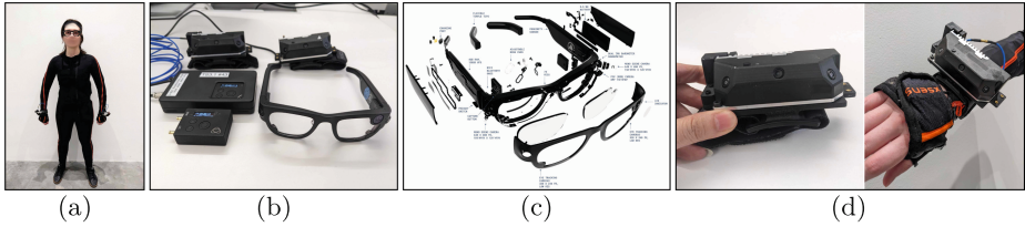
Fig. 2. Capture setup. (a) A full-dressed participant. (b) The set of hardware including Project Aria glasses, two miniAria wristbands and synchronization device. (c) The sensor suite of Project Aria and (d) the miniAria wristband.
